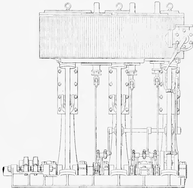
TRIPLE-EXPANSION ENGINE OF ISAAC BEARINGER'S STEAM YACHT WAPITI.
